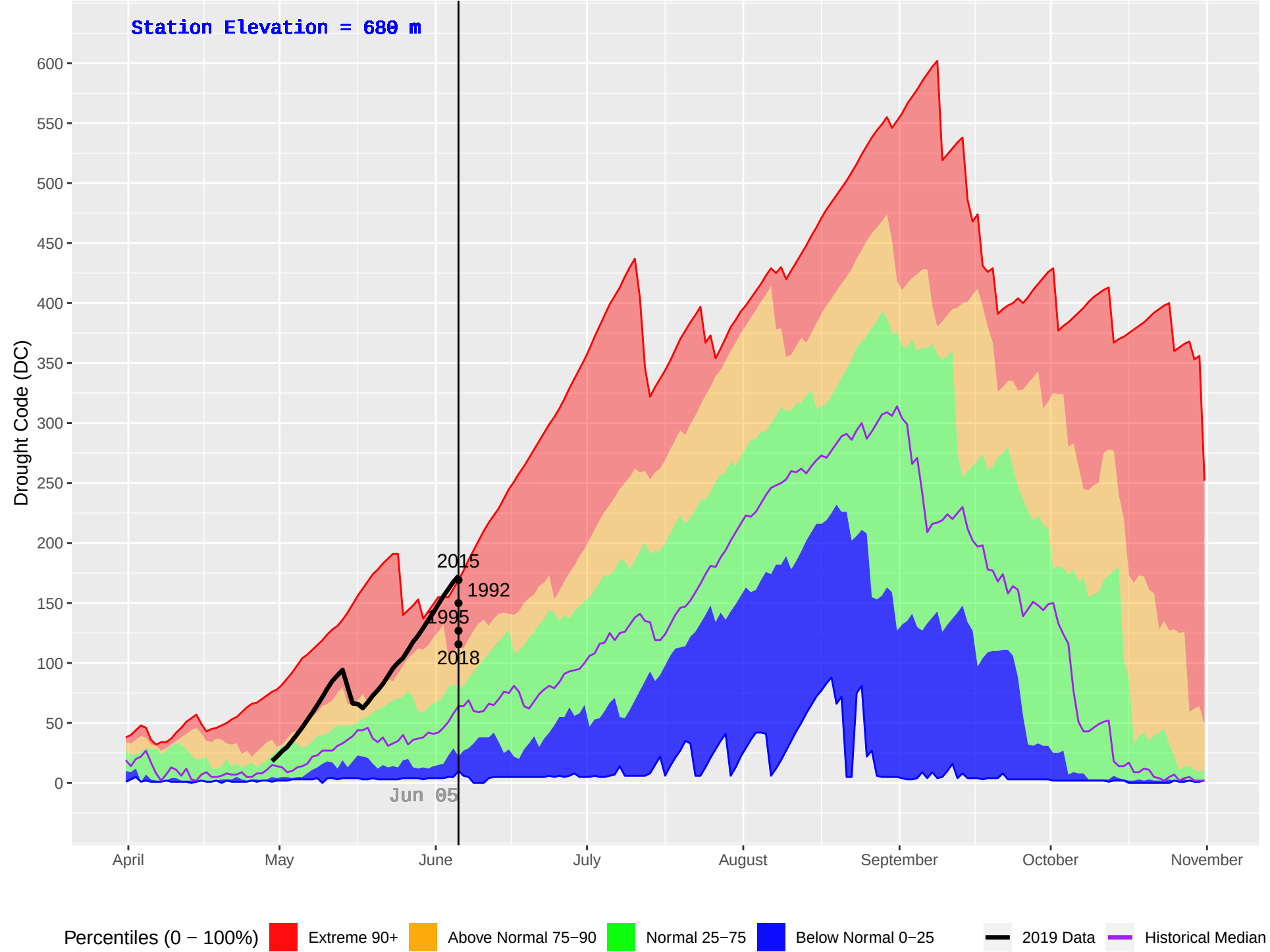
SUMMIT (11) : Historical (1985–2018) and Current (2019) Daily Drought Code (DC)
