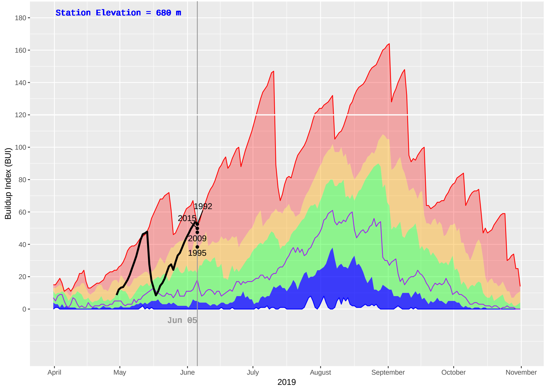
SUMMIT (11) : Historical (1985–2018), Current (2019) Daily Buildup Index (BUI)
