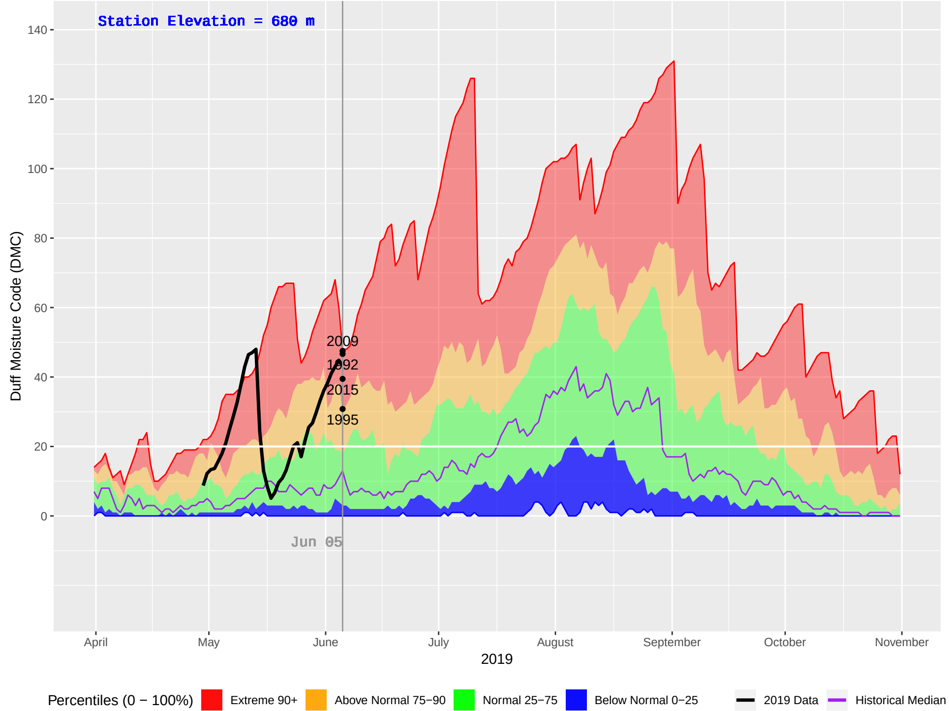
SUMMIT (11) : Historical (1985–2018), Current (2019) Daily Duff Moisture Code (DMC)
