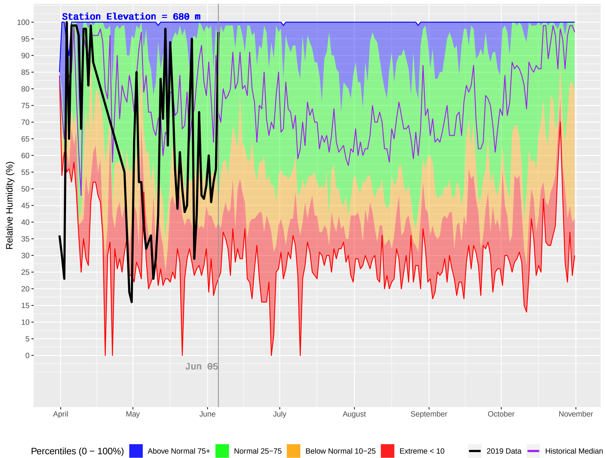
SUMMIT (11) : Historical (1985–2018) and Current (2019) Daily Relative Humidity
