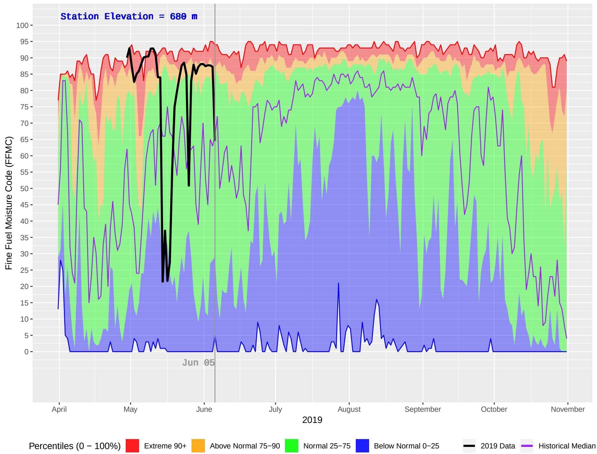
SUMMIT (11) : Historical (1985–2018) and Current (2019) Daily Fine Fuel Moisture Code (FFMC)
